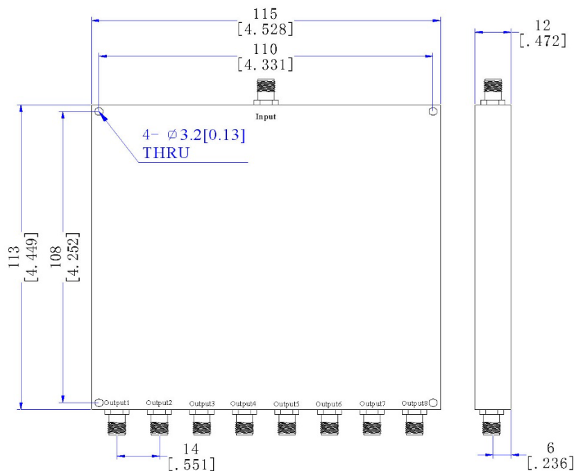
Dimensions (Unit: mm/[inch], Tolerance: \pm 0.3 mm)
